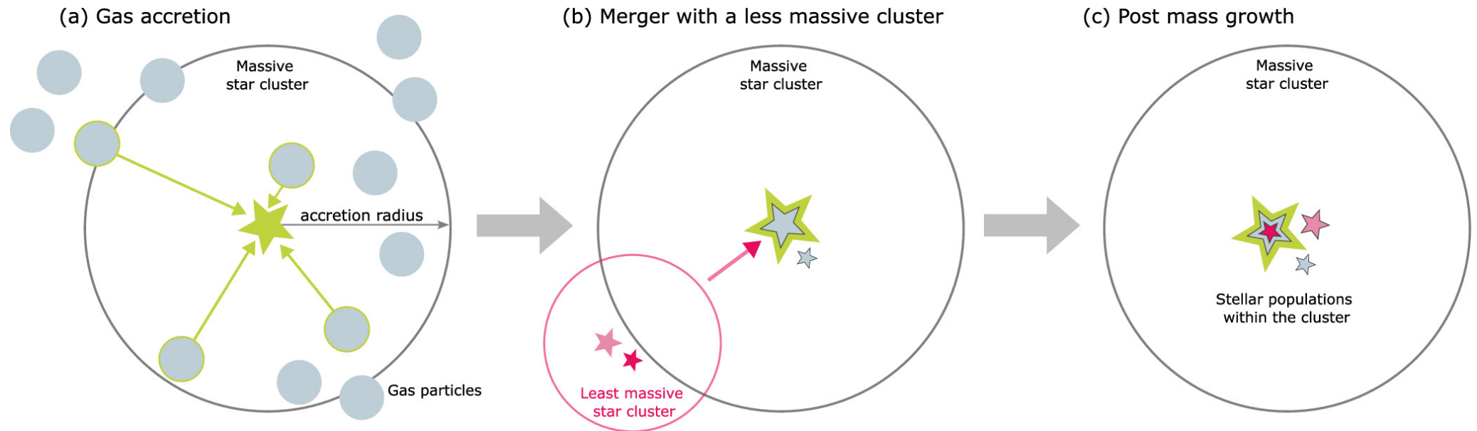
Figure 1. from Marta Reina-Campos et al 2025 Astrophys. J. 978 doi:10.3847/1538-4357/ad909f https://dx.doi.org/10.3847/1538-4357/ad909f © 2024. The Author(s). Published by the American Astronomical Society.
