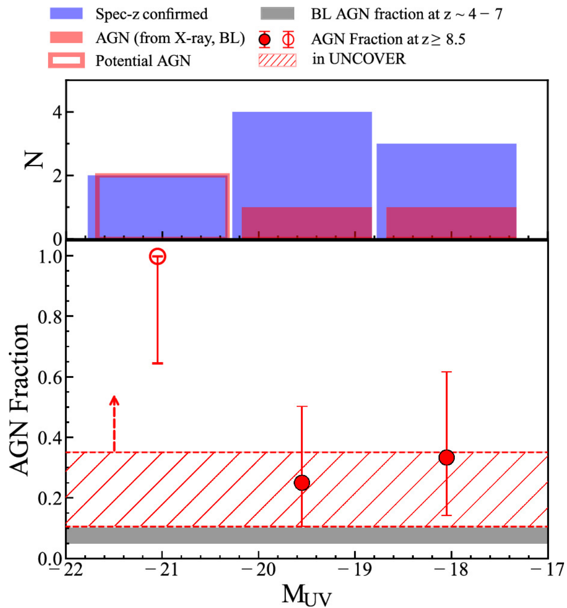
Figure 8. from Seiji Fujimoto et al 2024 Astrophys. J. 977 doi:10.3847/1538-4357/ad9027 https://dx.doi.org/10.3847/1538-4357/ad9027 © 2024. The Author(s). Published by the American Astronomical Society.
