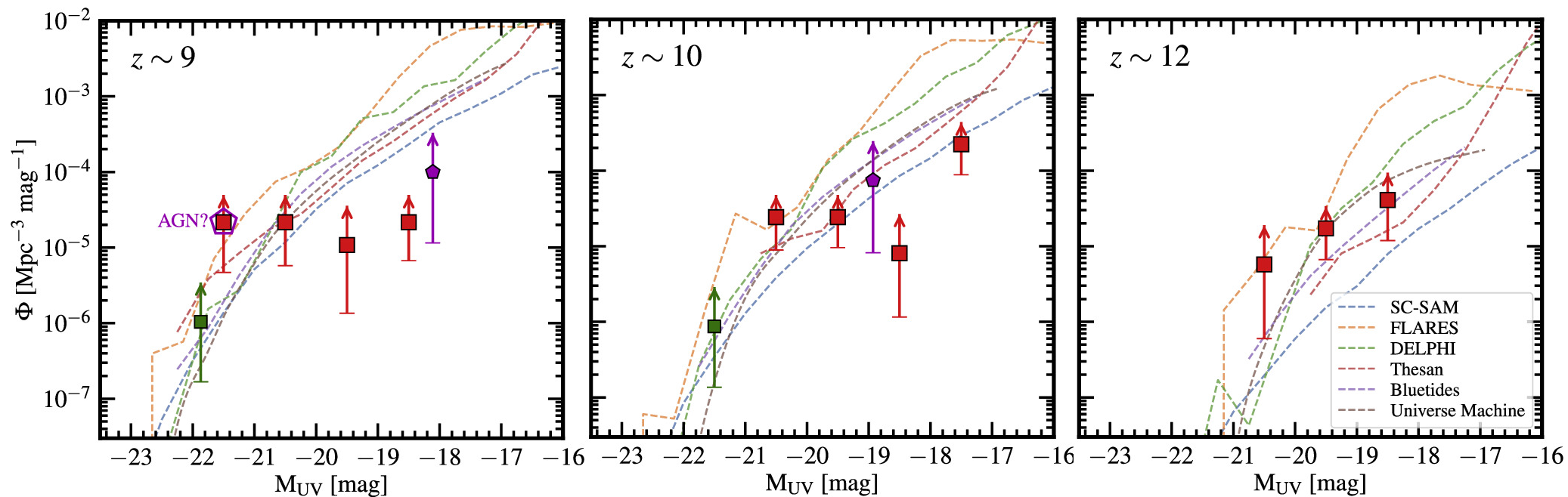
Figure 7. from Seiji Fujimoto et al 2024 Astrophys. J. 977 doi:10.3847/1538-4357/ad9027 https://dx.doi.org/10.3847/1538-4357/ad9027 © 2024. The Author(s). Published by the American Astronomical Society.
