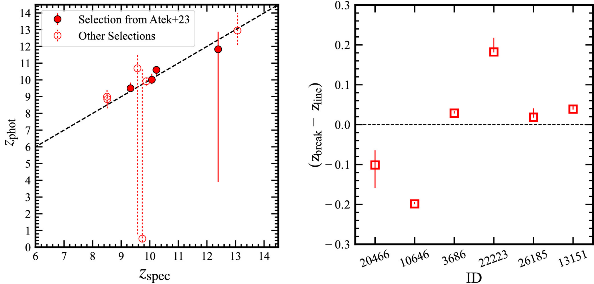
Figure 5. from Seiji Fujimoto et al 2024 Astrophys. J. 977 doi:10.3847/1538-4357/ad9027 https://dx.doi.org/10.3847/1538-4357/ad9027 © 2024. The Author(s). Published by the American Astronomical Society.
