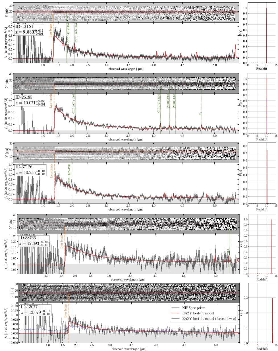
Figure 3. from Seiji Fujimoto et al 2024 Astrophys. J. 977 doi:10.3847/1538-4357/ad9027 https://dx.doi.org/10.3847/1538-4357/ad9027 © 2024. The Author(s). Published by the American Astronomical Society.
