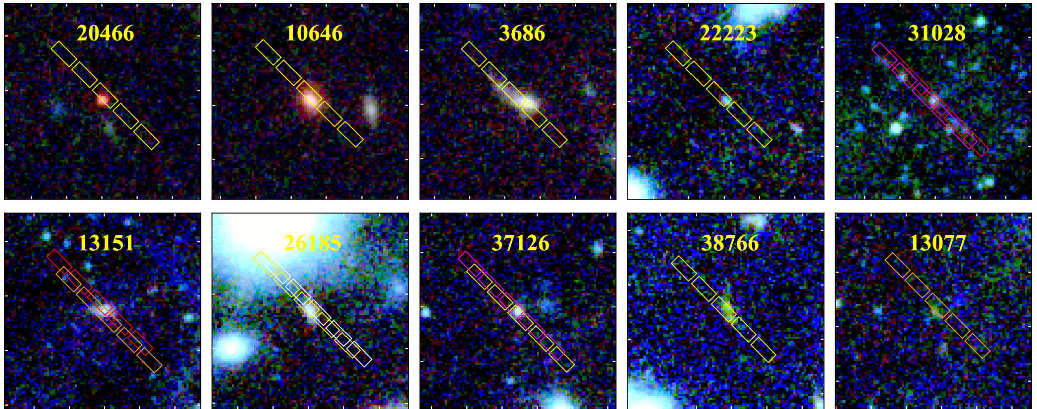
Figure 2. from Seiji Fujimoto et al 2024 Astrophys. J. 977 doi:10.3847/1538-4357/ad9027 https://dx.doi.org/10.3847/1538-4357/ad9027 © 2024. The Author(s). Published by the American Astronomical Society.
