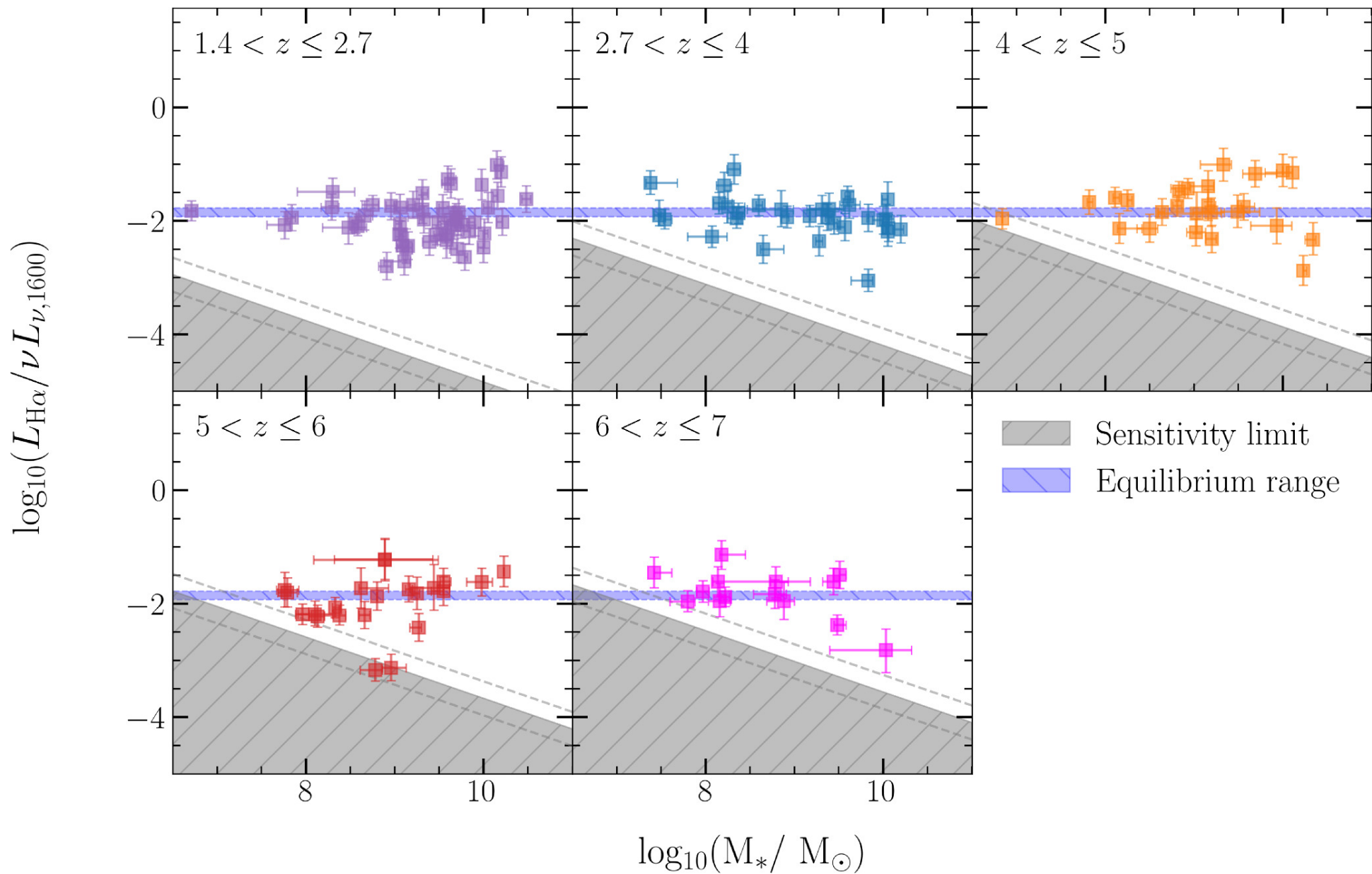
Figure 7. from Leonardo Clarke et al 2024 Astrophys. J. 977 doi:10.3847/1538-4357/ad8ba4 https://dx.doi.org/10.3847/1538-4357/ad8ba4 © 2024. The Author(s). Published by the American Astronomical Society.
