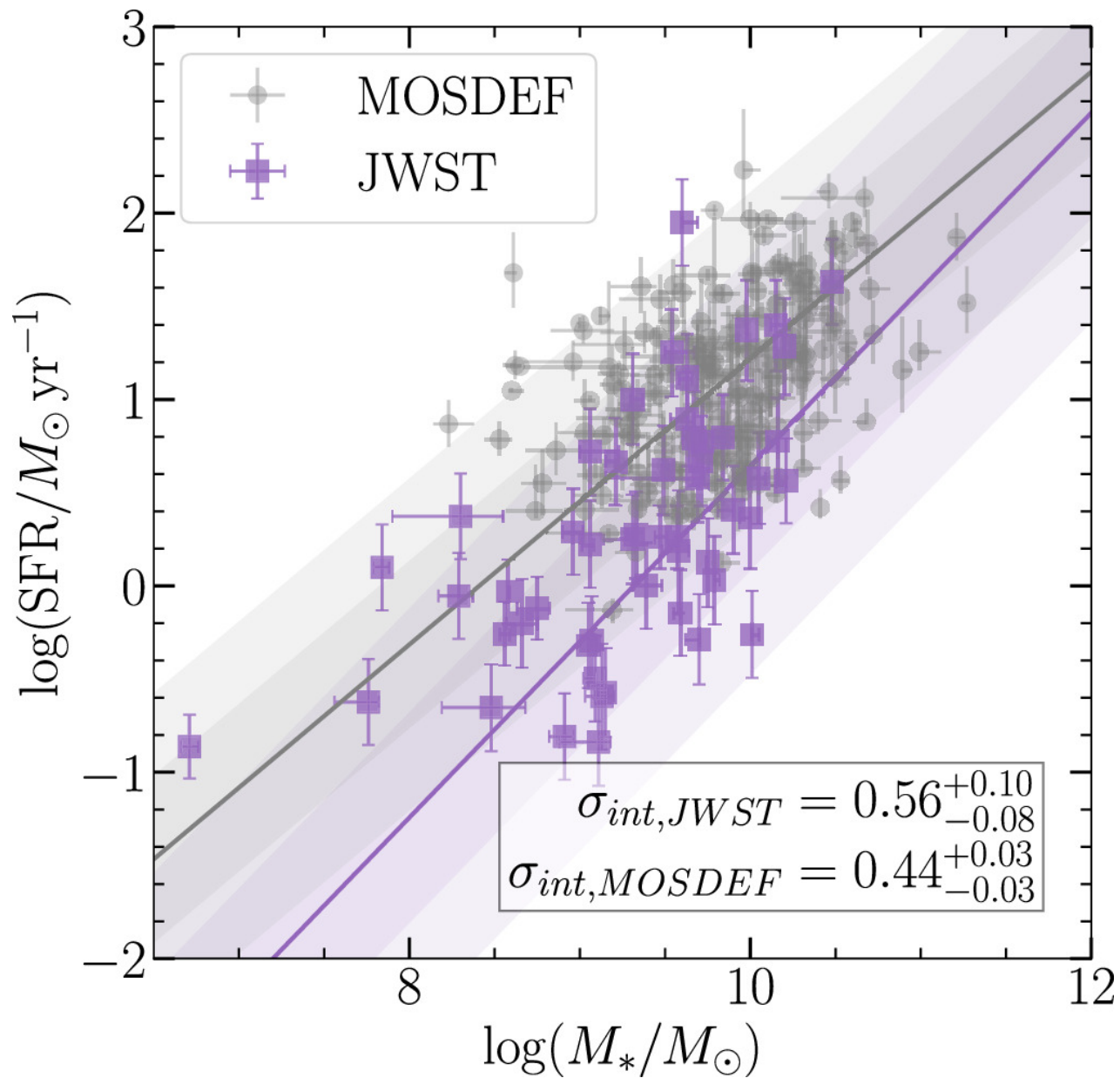
Figure 6. from Leonardo Clarke et al 2024 Astrophys. J. 977 doi:10.3847/1538-4357/ad8ba4 https://dx.doi.org/10.3847/1538-4357/ad8ba4 © 2024. The Author(s). Published by the American Astronomical Society.
