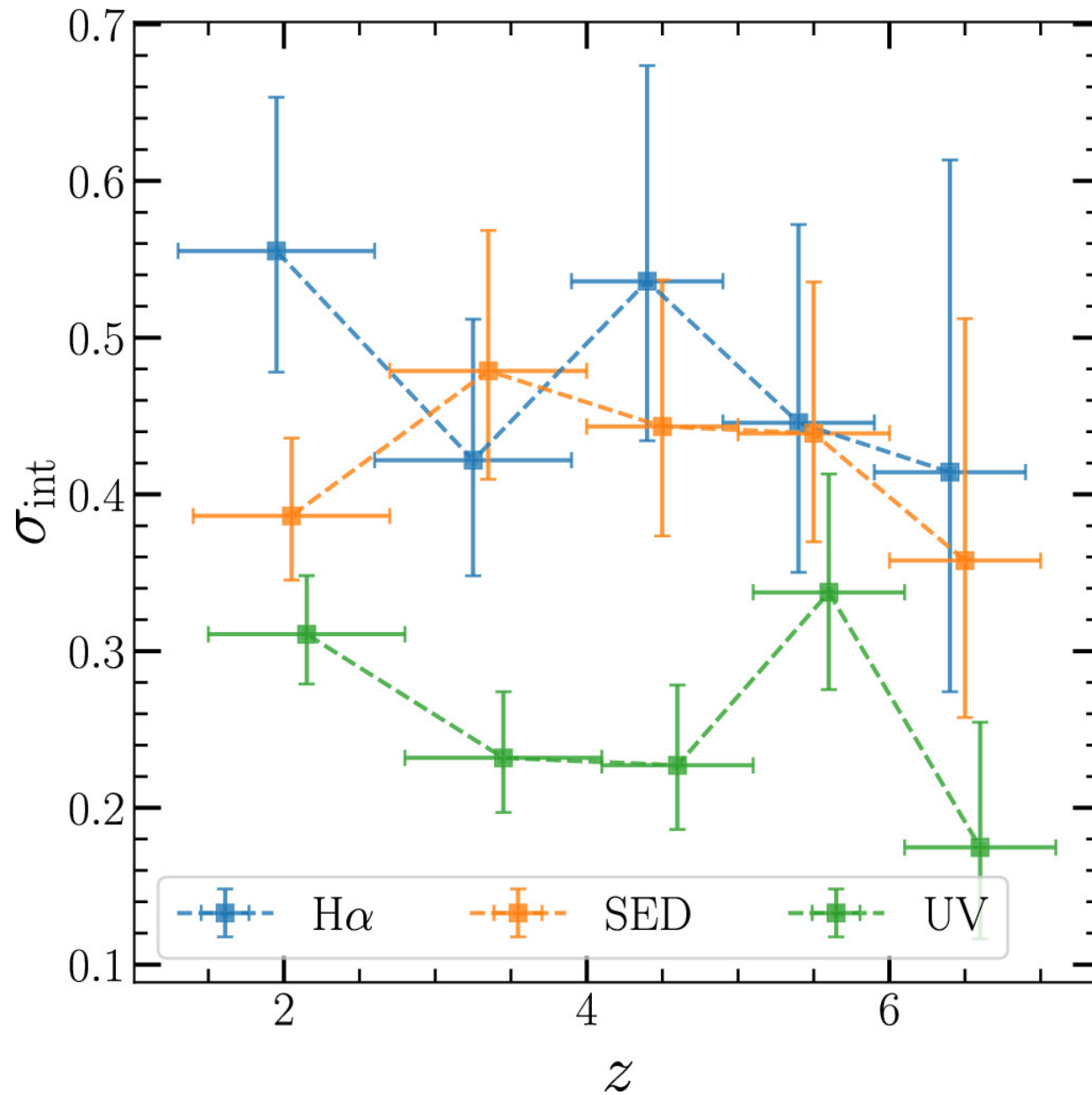
Figure 5. from Leonardo Clarke et al 2024 Astrophys. J. 977 doi:10.3847/1538-4357/ad8ba4 https://dx.doi.org/10.3847/1538-4357/ad8ba4 © 2024. The Author(s). Published by the American Astronomical Society.
