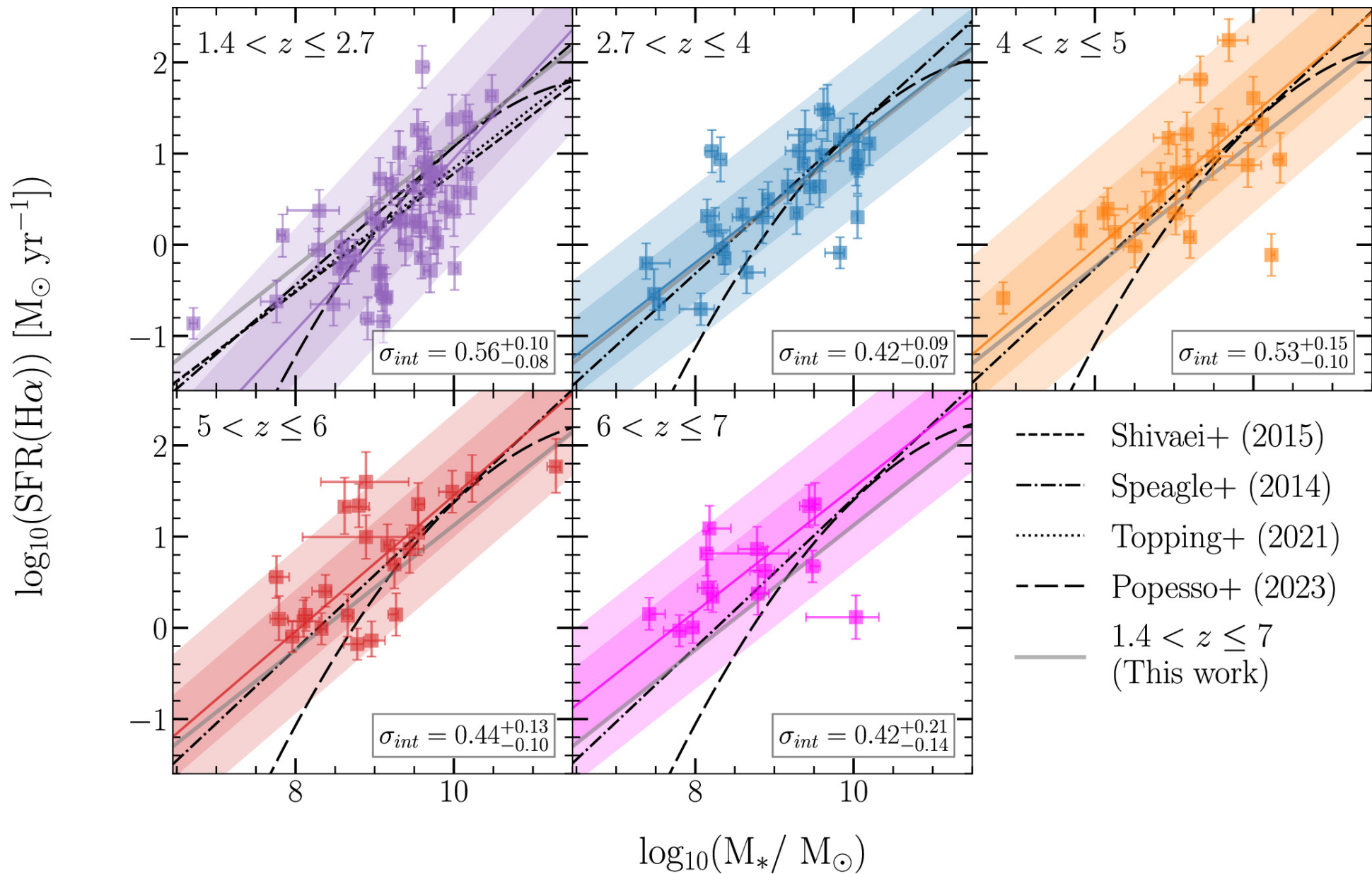
Figure 2. from Leonardo Clarke et al 2024 Astrophys. J. 977 doi:10.3847/1538-4357/ad8ba4 https://dx.doi.org/10.3847/1538-4357/ad8ba4 © 2024. The Author(s). Published by the American Astronomical Society.
