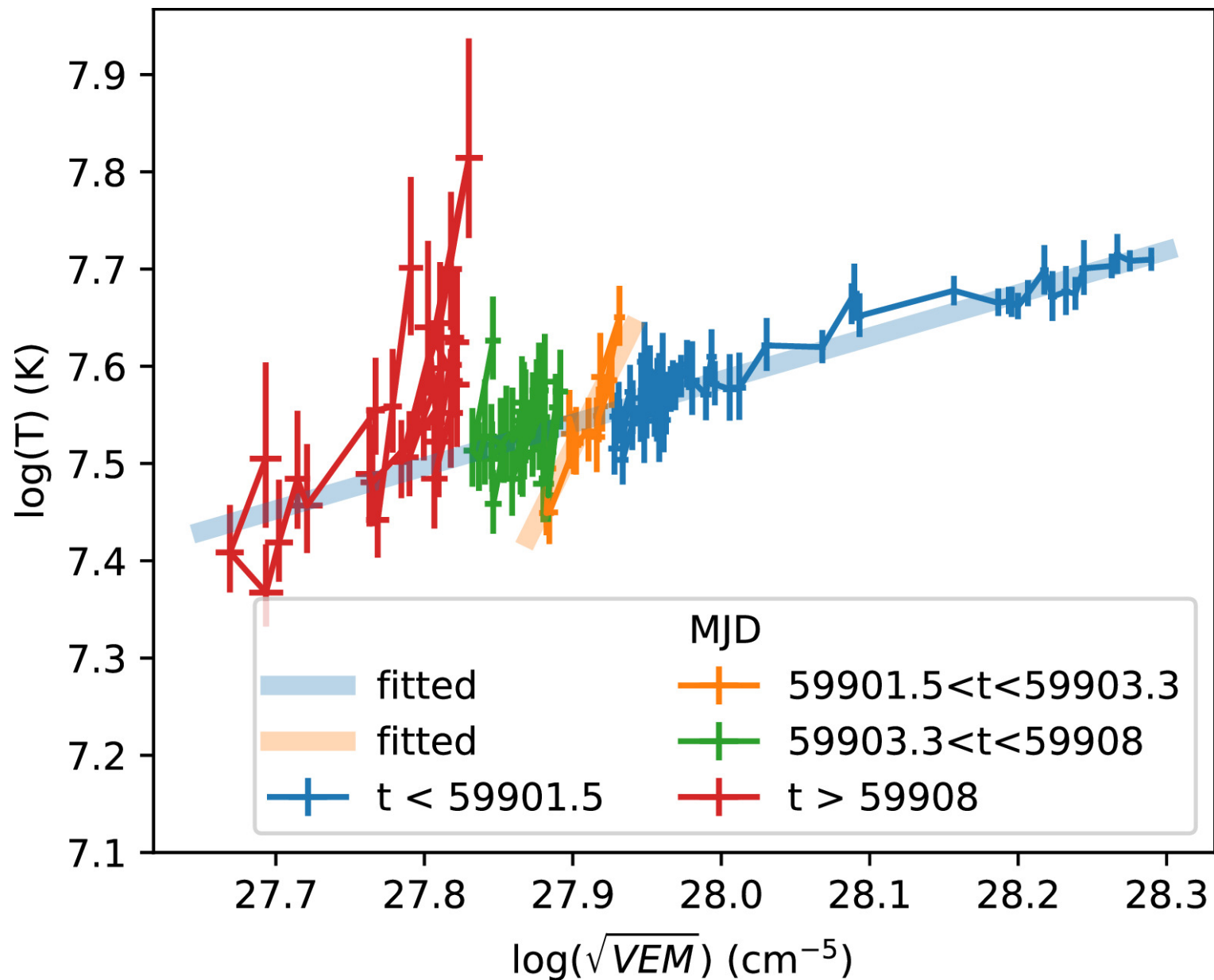
Figure 9. from Hans Moritz Günther et al 2024 Astrophys. J. 977 doi:10.3847/1538-4357/ad8b2c https://dx.doi.org/10.3847/1538-4357/ad8b2c © 2024. The Author(s). Published by the American Astronomical Society.
