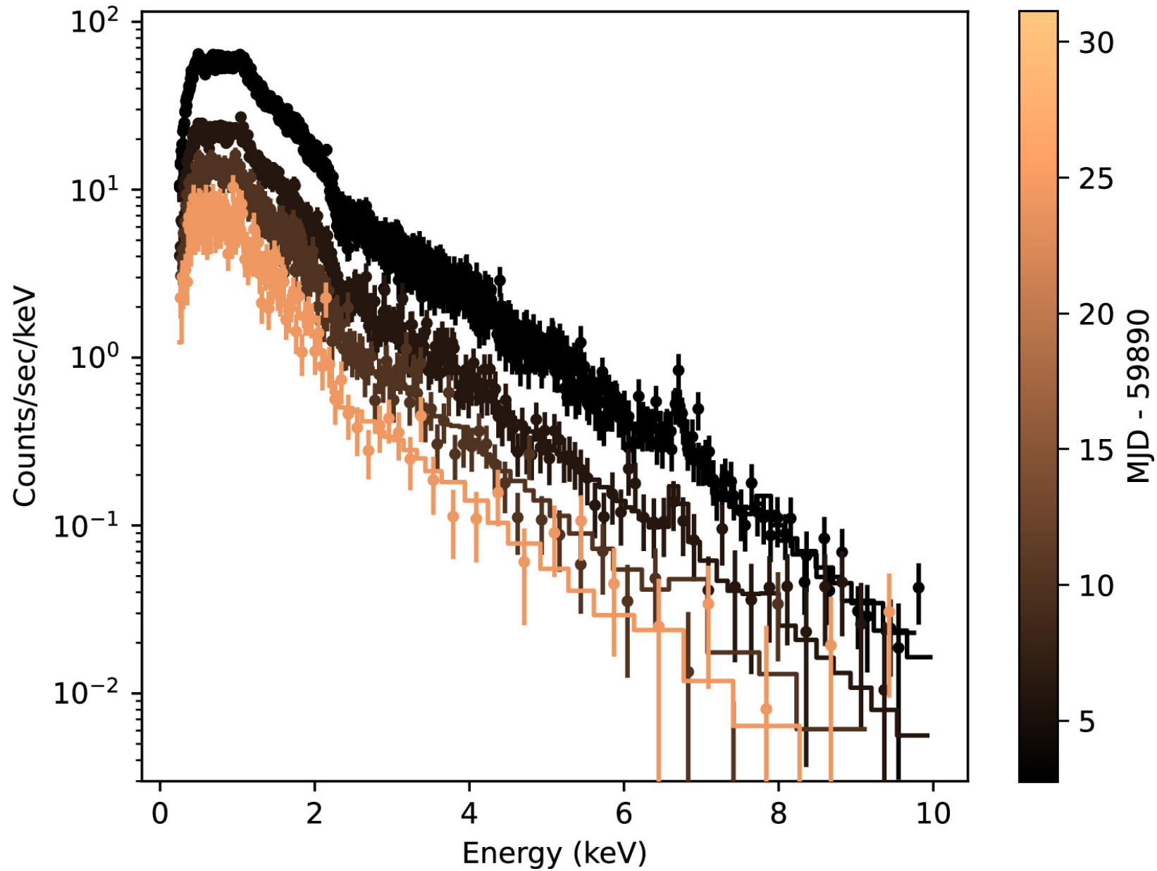
Figure 8. from Hans Moritz Günther et al 2024 Astrophys. J. 977 doi:10.3847/1538-4357/ad8b2c https://dx.doi.org/10.3847/1538-4357/ad8b2c © 2024. The Author(s). Published by the American Astronomical Society.
