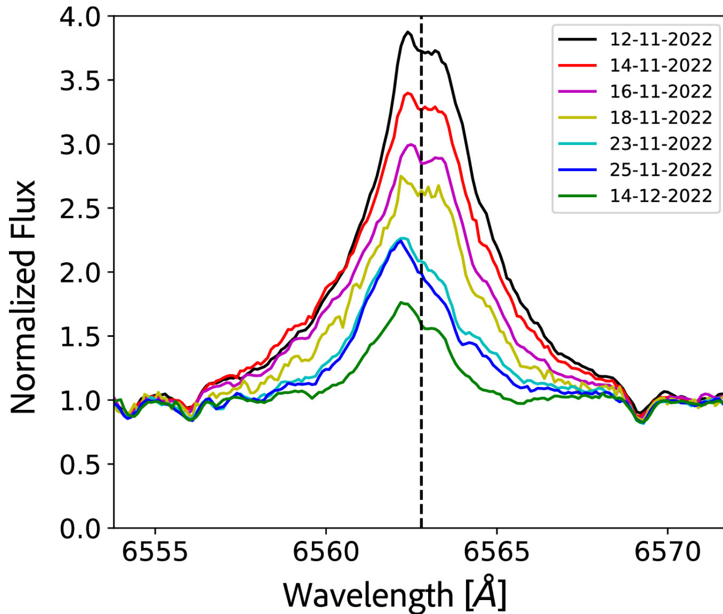
Figure 6. from Hans Moritz Günther et al 2024 Astrophys. J. 977 doi:10.3847/1538-4357/ad8b2c https://dx.doi.org/10.3847/1538-4357/ad8b2c © 2024. The Author(s). Published by the American Astronomical Society.
