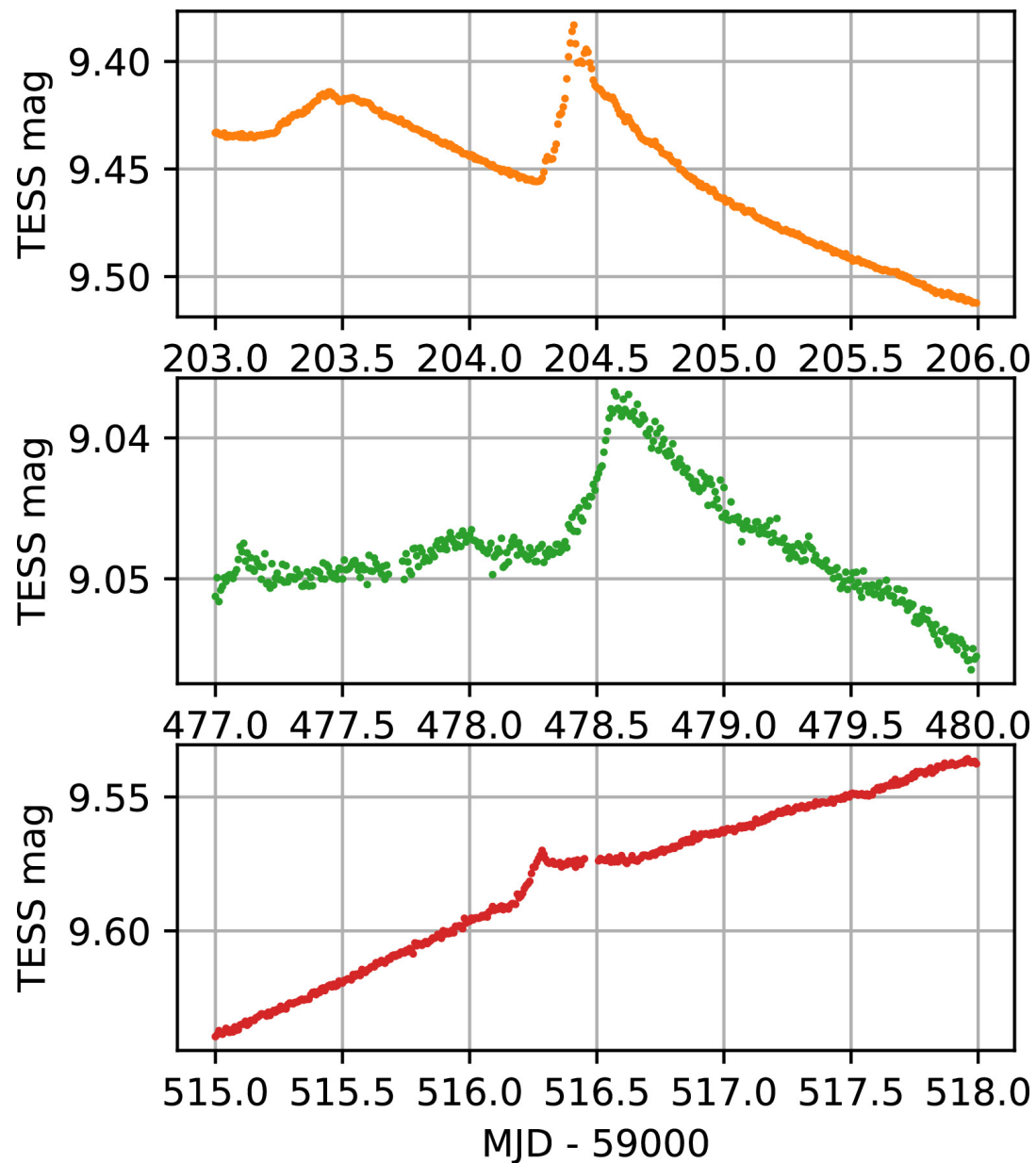
Figure 5. from Hans Moritz Günther et al 2024 Astrophys. J. 977 doi:10.3847/1538-4357/ad8b2c https://dx.doi.org/10.3847/1538-4357/ad8b2c © 2024. The Author(s). Published by the American Astronomical Society.
