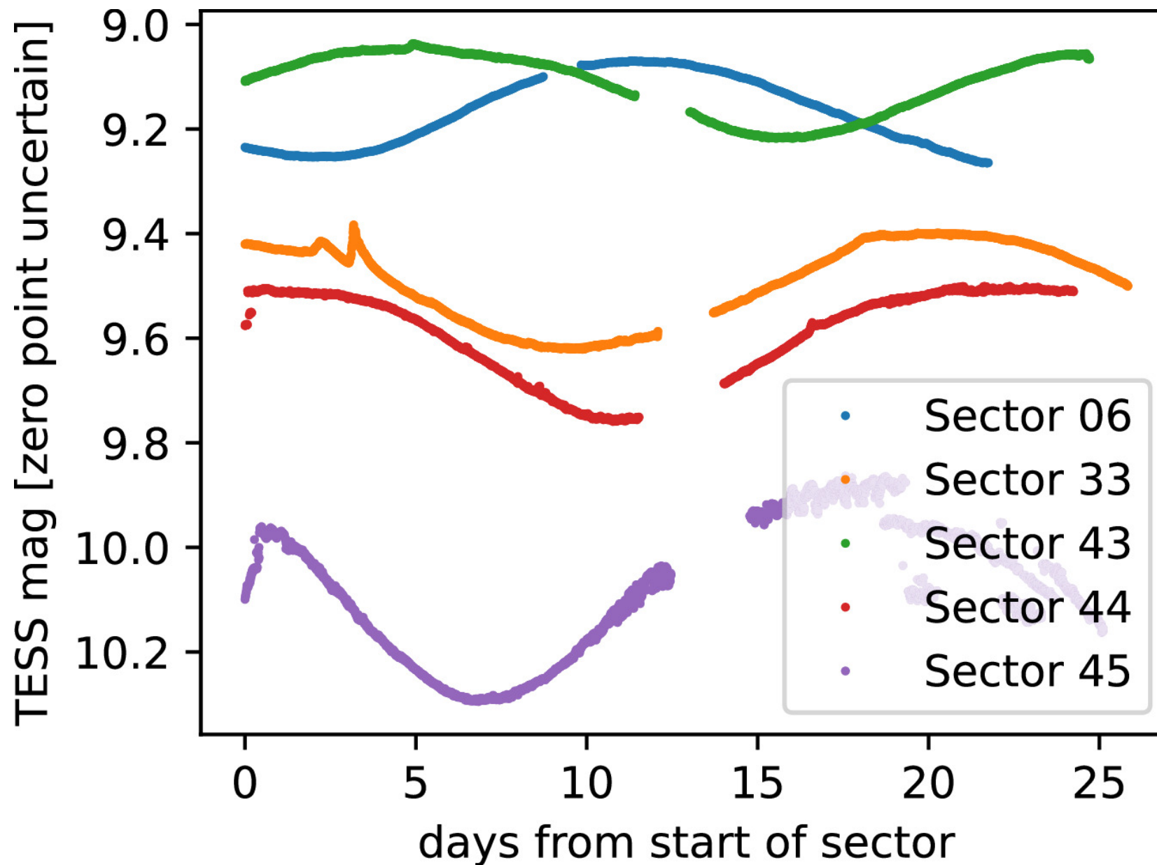
Figure 4. from Hans Moritz Günther et al 2024 Astrophys. J. 977 doi:10.3847/1538-4357/ad8b2c https://dx.doi.org/10.3847/1538-4357/ad8b2c © 2024. The Author(s). Published by the American Astronomical Society.
