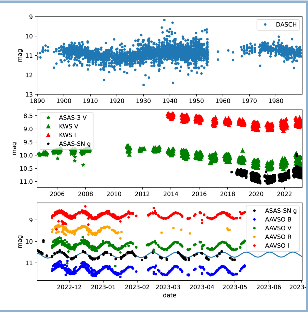
Figure 2. from Hans Moritz Günther et al 2024 Astrophys. J. 977 doi:10.3847/1538-4357/ad8b2c https://dx.doi.org/10.3847/1538-4357/ad8b2c © 2024. The Author(s). Published by the American Astronomical Society.
