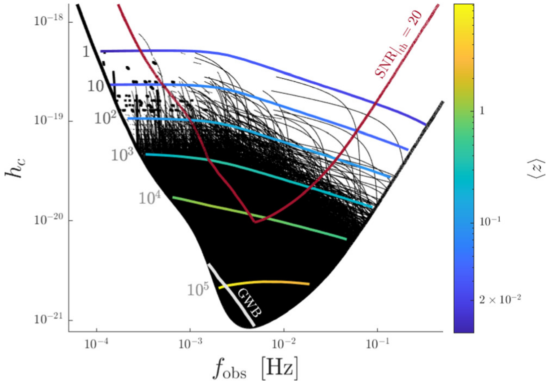
Figure 6. from Barak Rom et al 2024 Astrophys. J. 977 doi:10.3847/1538-4357/ad8b1d https://dx.doi.org/10.3847/1538-4357/ad8b1d © 2024. The Author(s). Published by the American Astronomical Society.
