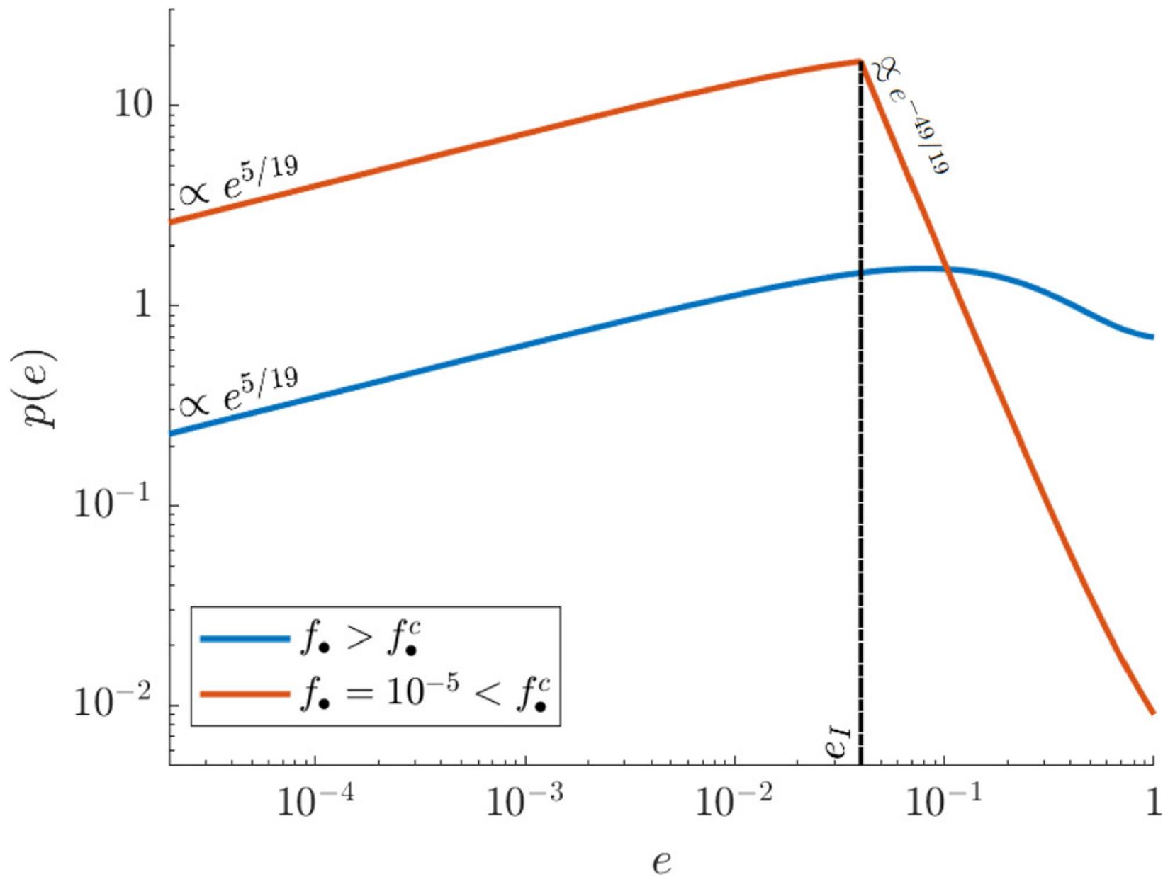
Figure 4. from Barak Rom et al 2024 Astrophys. J. 977 doi:10.3847/1538-4357/ad8b1d https://dx.doi.org/10.3847/1538-4357/ad8b1d © 2024. The Author(s). Published by the American Astronomical Society.
