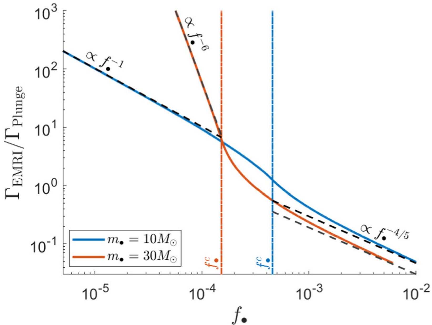
Figure 3. from Barak Rom et al 2024 Astrophys. J. 977 doi:10.3847/1538-4357/ad8b1d https://dx.doi.org/10.3847/1538-4357/ad8b1d © 2024. The Author(s). Published by the American Astronomical Society.
