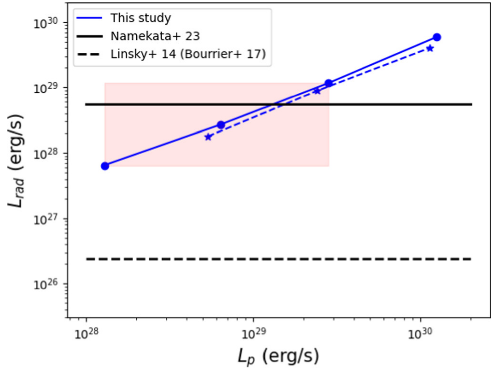
Figure 9. from Victor Réville et al 2024 Astrophys. J. 976 doi:10.3847/1538-4357/ad8132 https://dx.doi.org/10.3847/1538-4357/ad8132 © 2024. The Author(s). Published by the American Astronomical Society.
