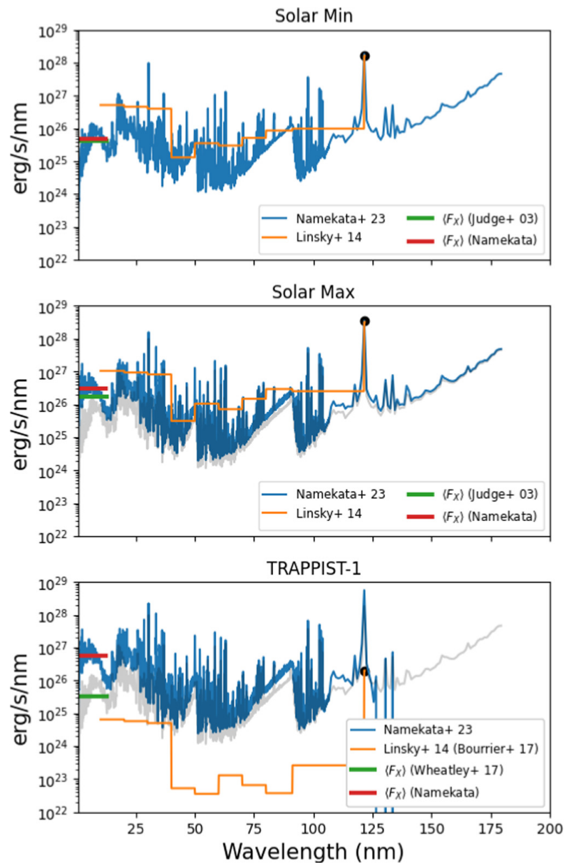
Figure 8. from Victor Réville et al 2024 Astrophys. J. 976 doi:10.3847/1538-4357/ad8132 https://dx.doi.org/10.3847/1538-4357/ad8132 © 2024. The Author(s). Published by the American Astronomical Society.
