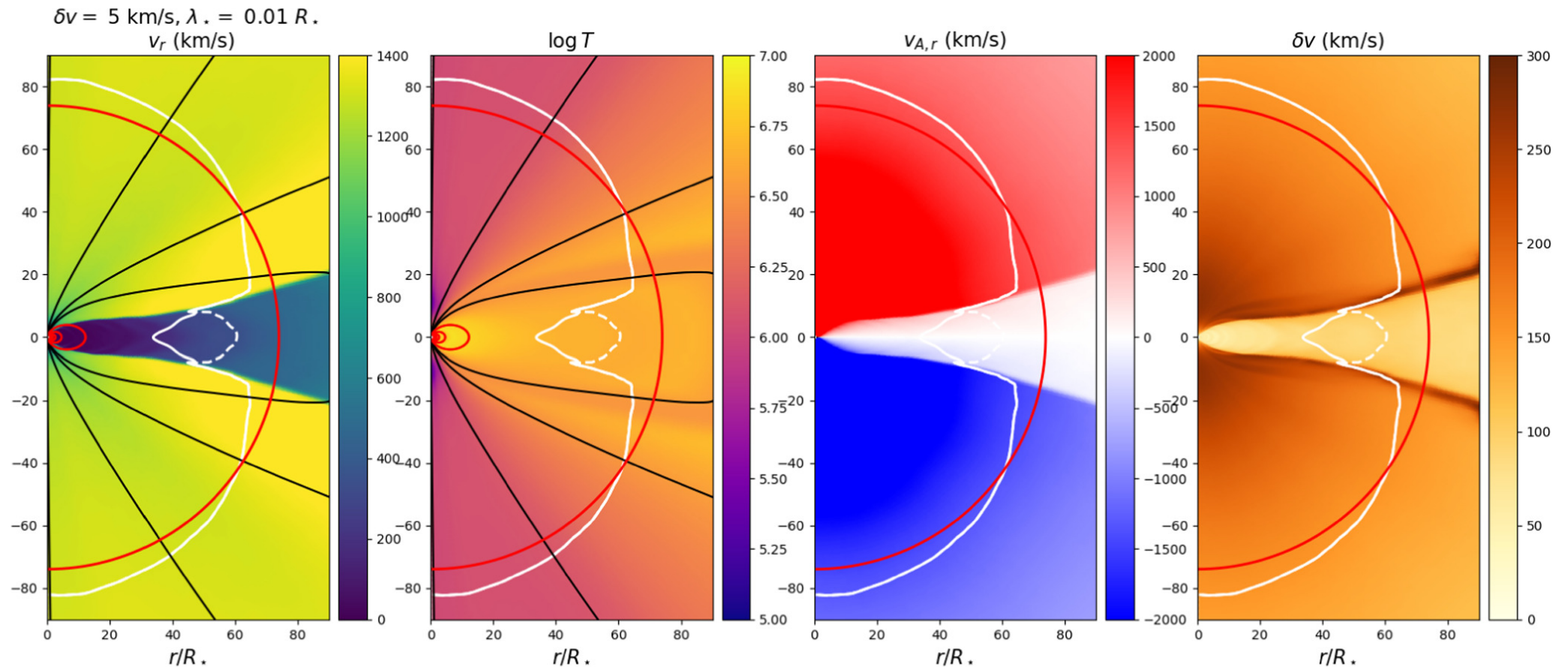
Figure 7. from Victor Réville et al 2024 Astrophys. J. 976 doi:10.3847/1538-4357/ad8132 https://dx.doi.org/10.3847/1538-4357/ad8132 © 2024. The Author(s). Published by the American Astronomical Society.
