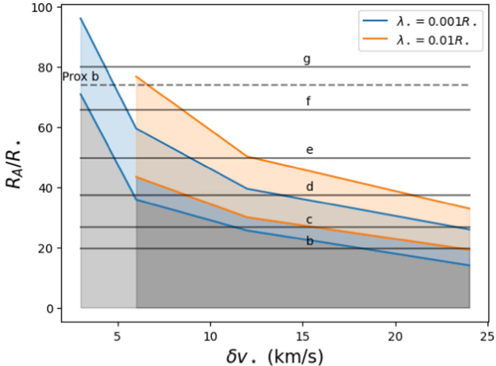
Figure 6. from Victor Réville et al 2024 Astrophys. J. 976 doi:10.3847/1538-4357/ad8132 https://dx.doi.org/10.3847/1538-4357/ad8132 © 2024. The Author(s). Published by the American Astronomical Society.
