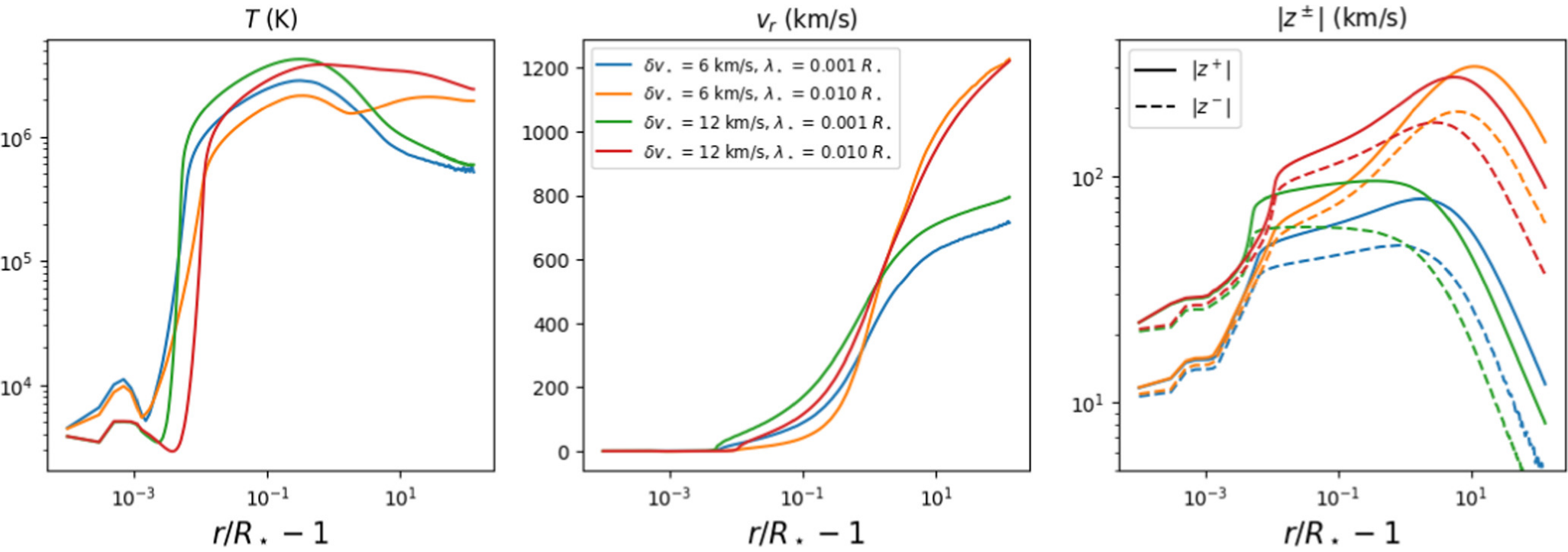
Figure 2. from Victor Réville et al 2024 Astrophys. J. 976 doi:10.3847/1538-4357/ad8132 https://dx.doi.org/10.3847/1538-4357/ad8132 © 2024. The Author(s). Published by the American Astronomical Society.
