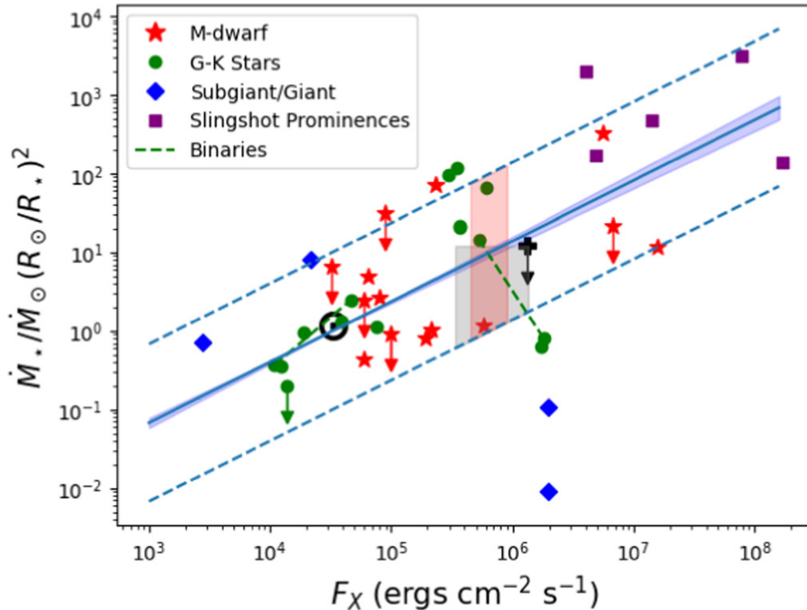
Figure 1. from Victor Réville et al 2024 Astrophys. J. 976 doi:10.3847/1538-4357/ad8132 https://dx.doi.org/10.3847/1538-4357/ad8132 © 2024. The Author(s). Published by the American Astronomical Society.
