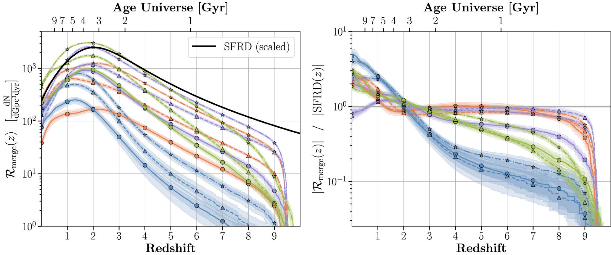
Figure 9. from Adam P. Boesky et al 2024 Astrophys. J. 976 doi:10.3847/1538-4357/ad7fe4 https://dx.doi.org/10.3847/1538-4357/ad7fe4 © 2024. The Author(s). Published by the American Astronomical Society.
