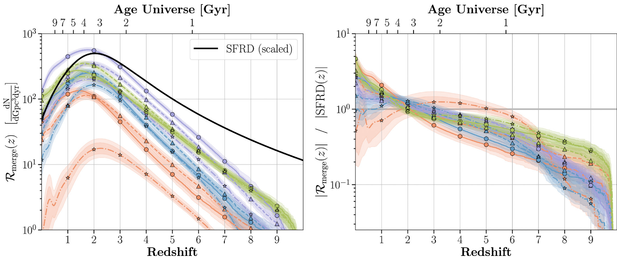
Figure 8. from Adam P. Boesky et al 2024 Astrophys. J. 976 doi:10.3847/1538-4357/ad7fe4 https://dx.doi.org/10.3847/1538-4357/ad7fe4 © 2024. The Author(s). Published by the American Astronomical Society.
