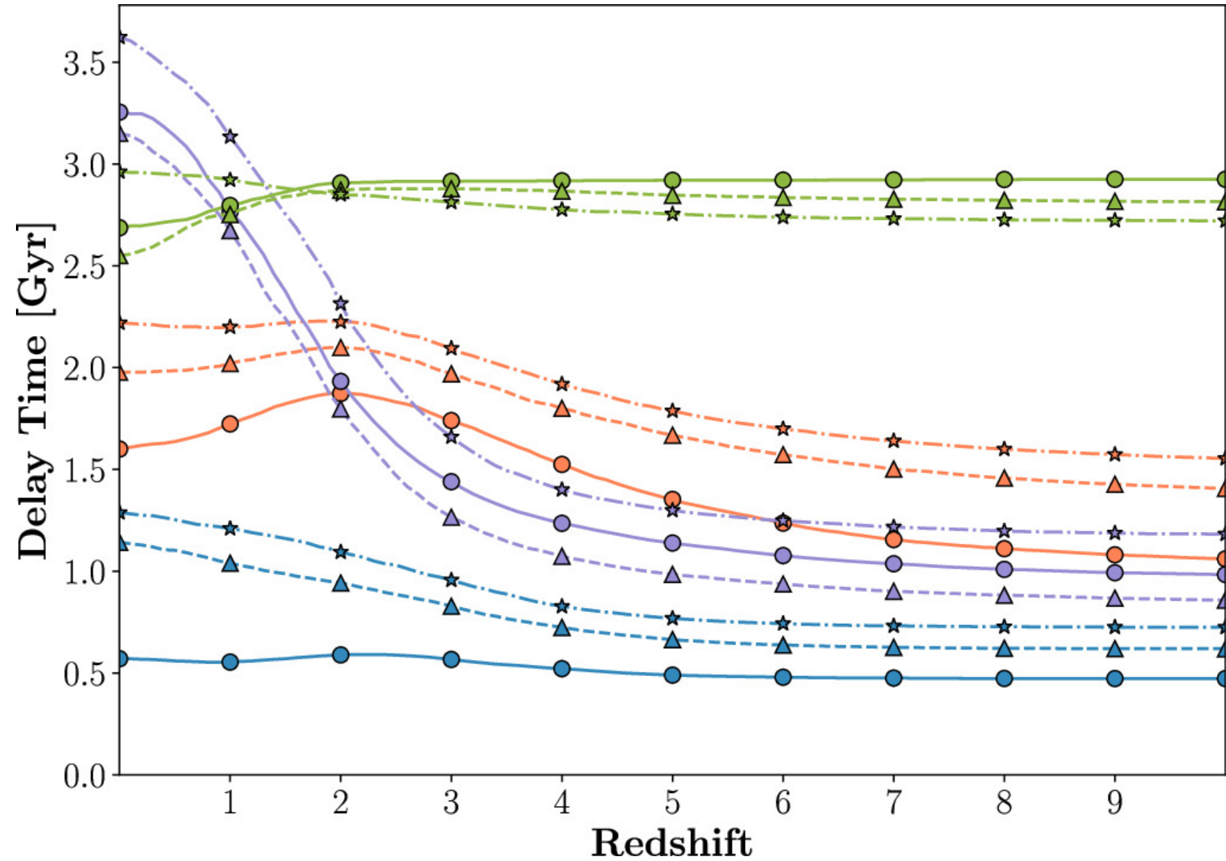
Figure 5. from Adam P. Boesky et al 2024 Astrophys. J. 976 doi:10.3847/1538-4357/ad7fe4 https://dx.doi.org/10.3847/1538-4357/ad7fe4 © 2024. The Author(s). Published by the American Astronomical Society.
