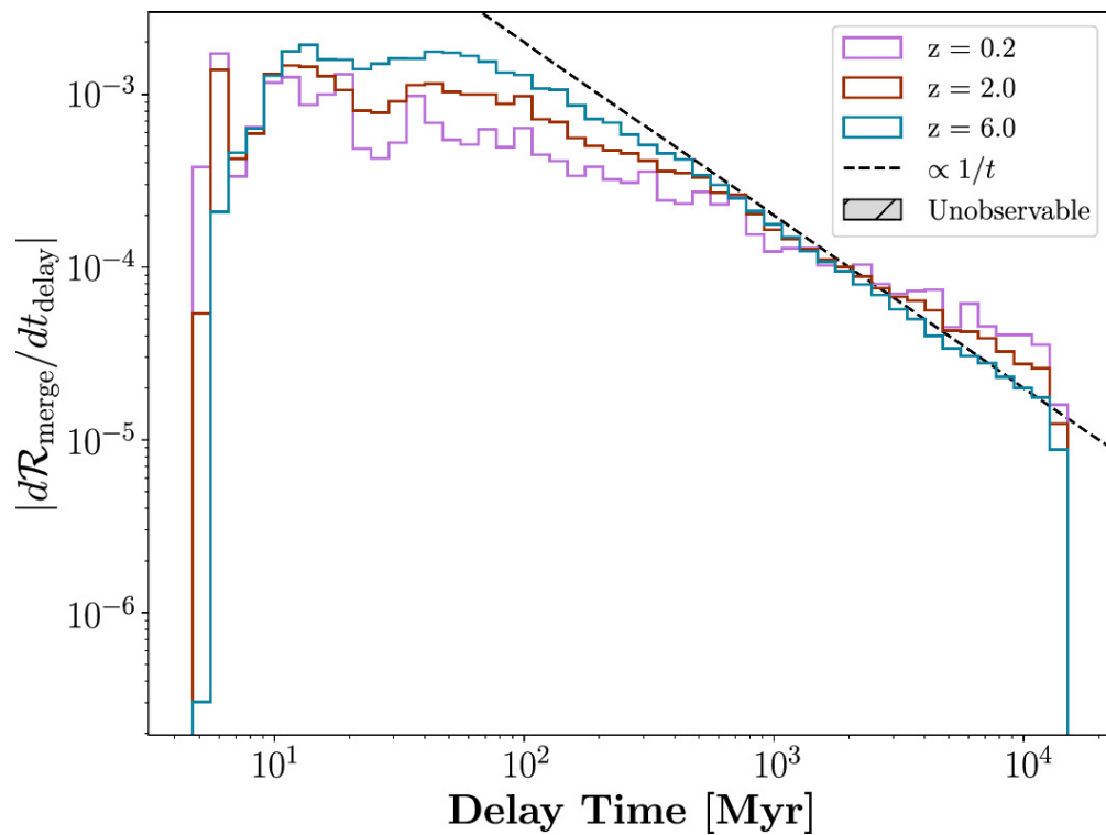
Figure 4. from Adam P. Boesky et al 2024 Astrophys. J. 976 doi:10.3847/1538-4357/ad7fe4 https://dx.doi.org/10.3847/1538-4357/ad7fe4 © 2024. The Author(s). Published by the American Astronomical Society.
