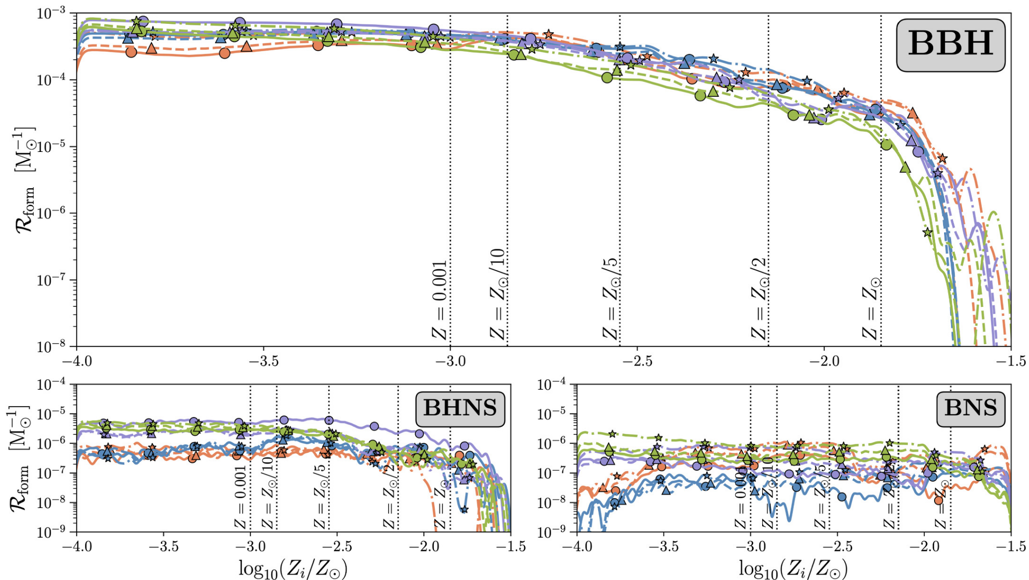
Figure 3. from Adam P. Boesky et al 2024 Astrophys. J. 976 doi:10.3847/1538-4357/ad7fe4 https://dx.doi.org/10.3847/1538-4357/ad7fe4 © 2024. The Author(s). Published by the American Astronomical Society.
