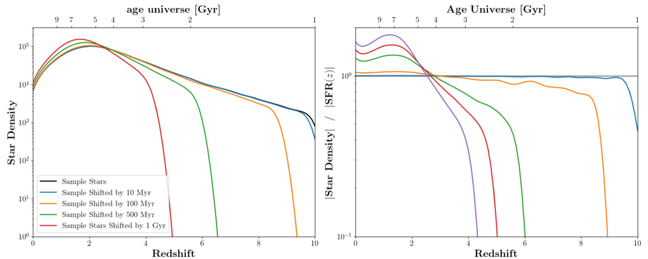
Figure 12. from Adam P. Boesky et al 2024 Astrophys. J. 976 doi:10.3847/1538-4357/ad7fe4 https://dx.doi.org/10.3847/1538-4357/ad7fe4 © 2024. The Author(s). Published by the American Astronomical Society.
