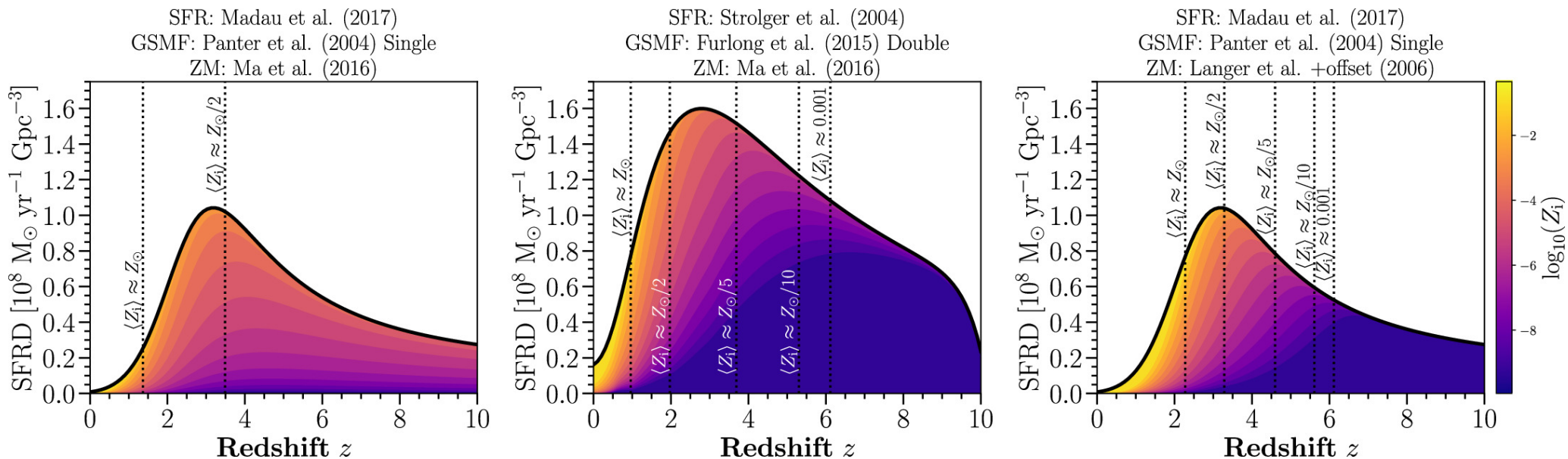
Figure 11. from Adam P. Boesky et al 2024 Astrophys. J. 976 doi:10.3847/1538-4357/ad7fe4 https://dx.doi.org/10.3847/1538-4357/ad7fe4 © 2024. The Author(s). Published by the American Astronomical Society.
