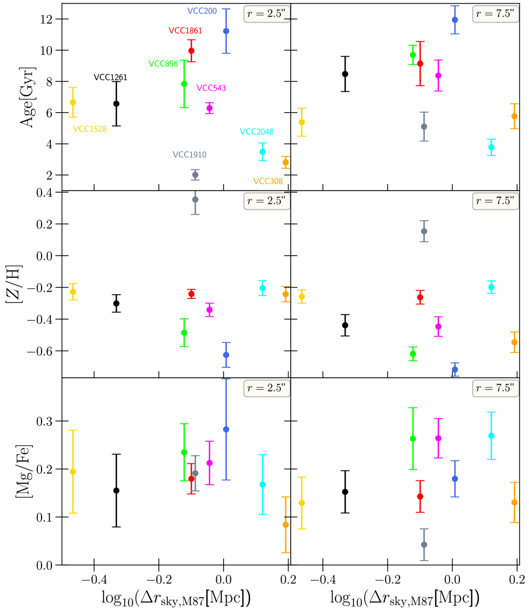
Figure 9. from Mathias Lipka et al 2024 Astrophys. J. 976 doi:10.3847/1538-4357/ad7bac https://dx.doi.org/10.3847/1538-4357/ad7bac © 2024. The Author(s). Published by the American Astronomical Society.
