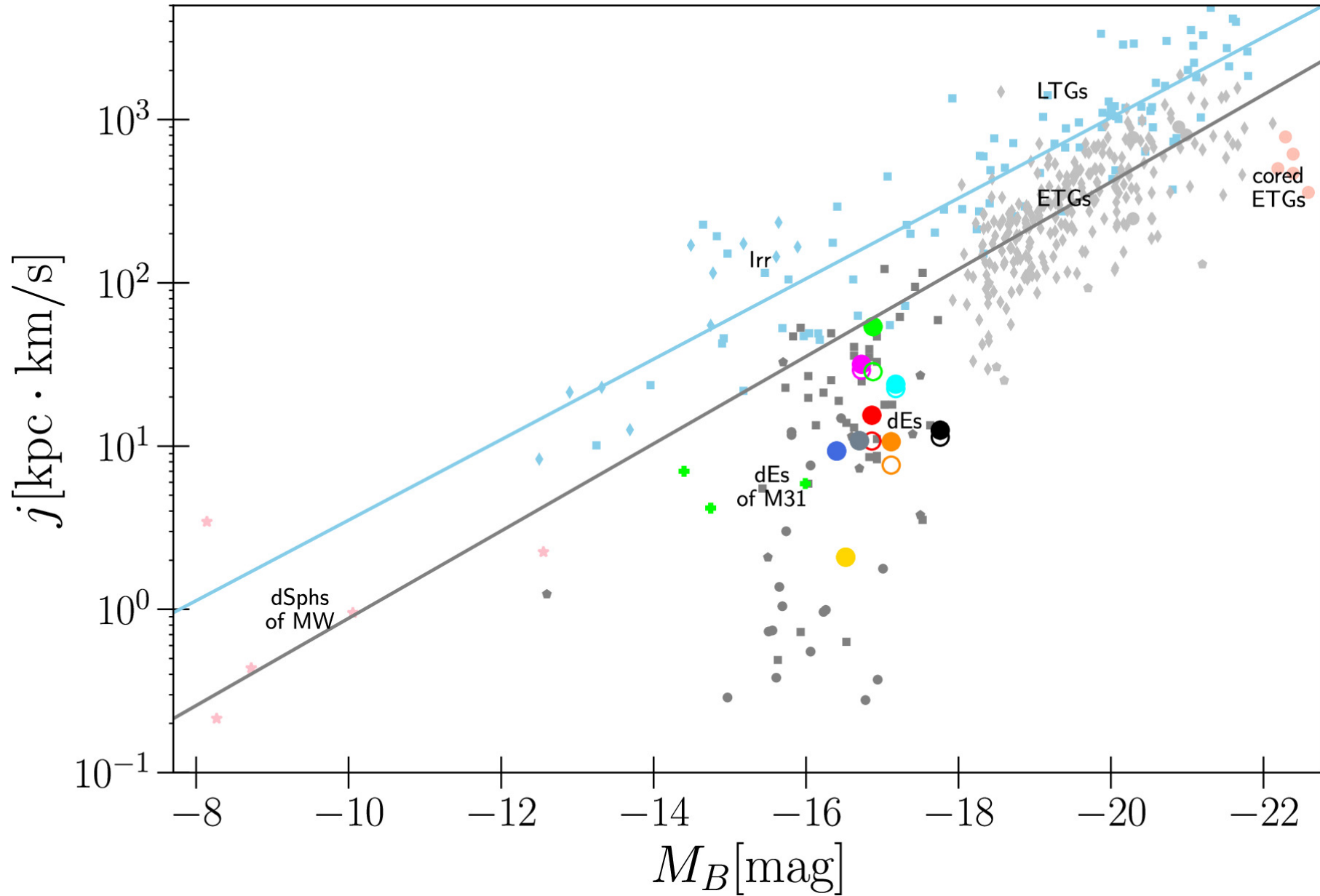
Figure 7. from Mathias Lipka et al 2024 Astrophys. J. 976 doi:10.3847/1538-4357/ad7bac https://dx.doi.org/10.3847/1538-4357/ad7bac © 2024. The Author(s). Published by the American Astronomical Society.
