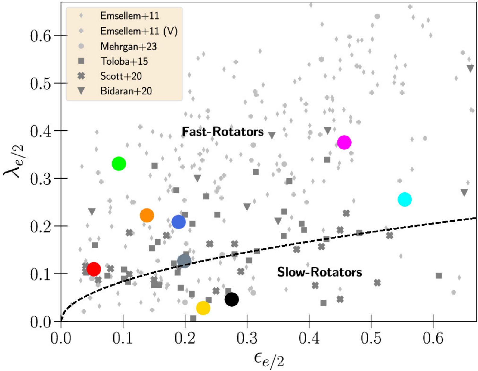
Figure 6. from Mathias Lipka et al 2024 Astrophys. J. 976 doi:10.3847/1538-4357/ad7bac https://dx.doi.org/10.3847/1538-4357/ad7bac © 2024. The Author(s). Published by the American Astronomical Society.
