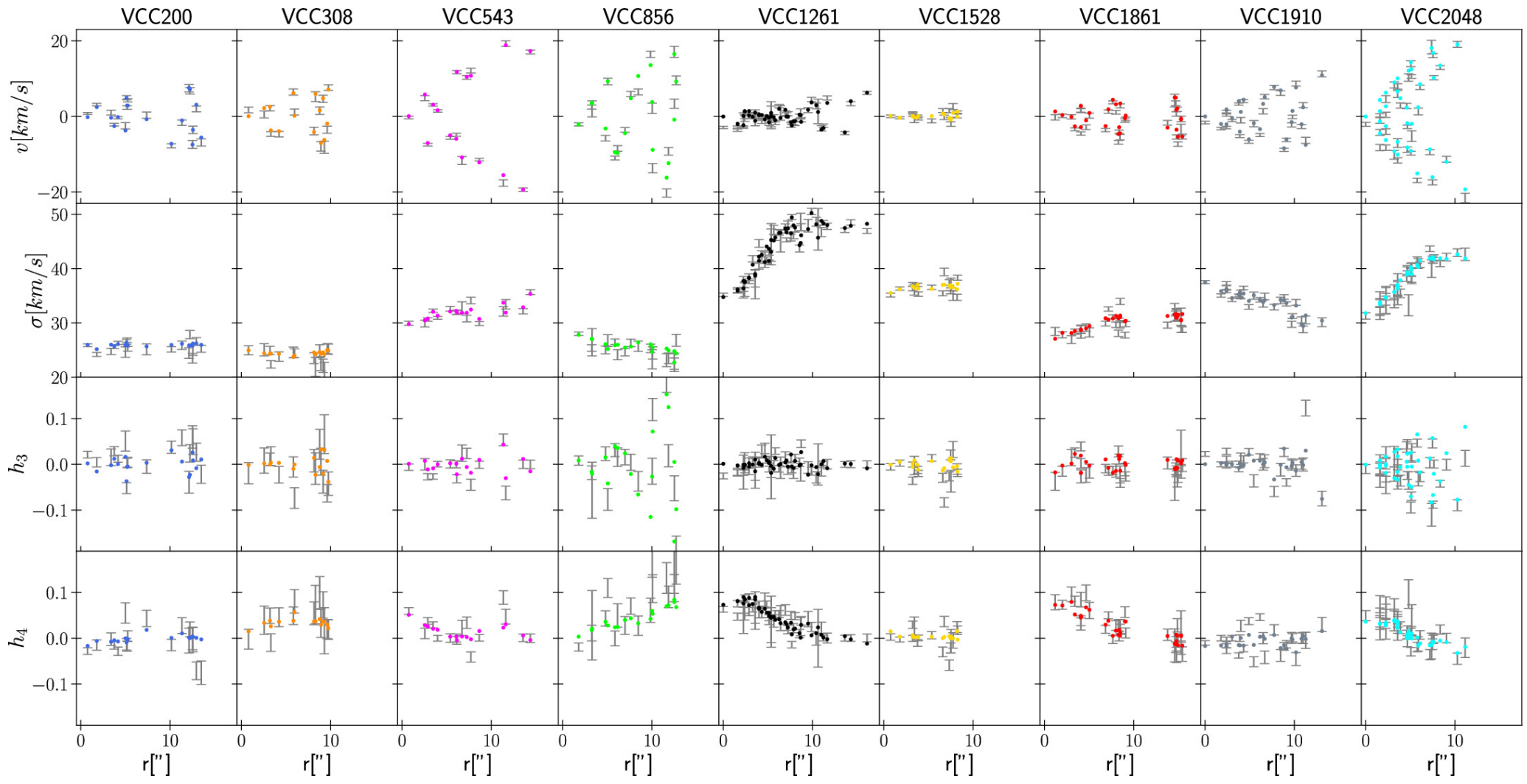
Figure 4. from Mathias Lipka et al 2024 Astrophys. J. 976 doi:10.3847/1538-4357/ad7bac https://dx.doi.org/10.3847/1538-4357/ad7bac © 2024. The Author(s). Published by the American Astronomical Society.
