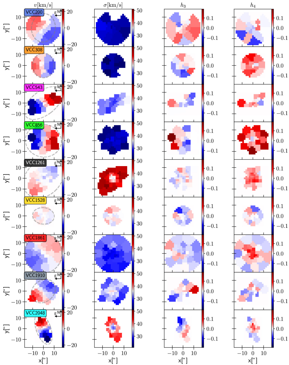
Figure 3. from Mathias Lipka et al 2024 Astrophys. J. 976 doi:10.3847/1538-4357/ad7bac https://dx.doi.org/10.3847/1538-4357/ad7bac © 2024. The Author(s). Published by the American Astronomical Society.
