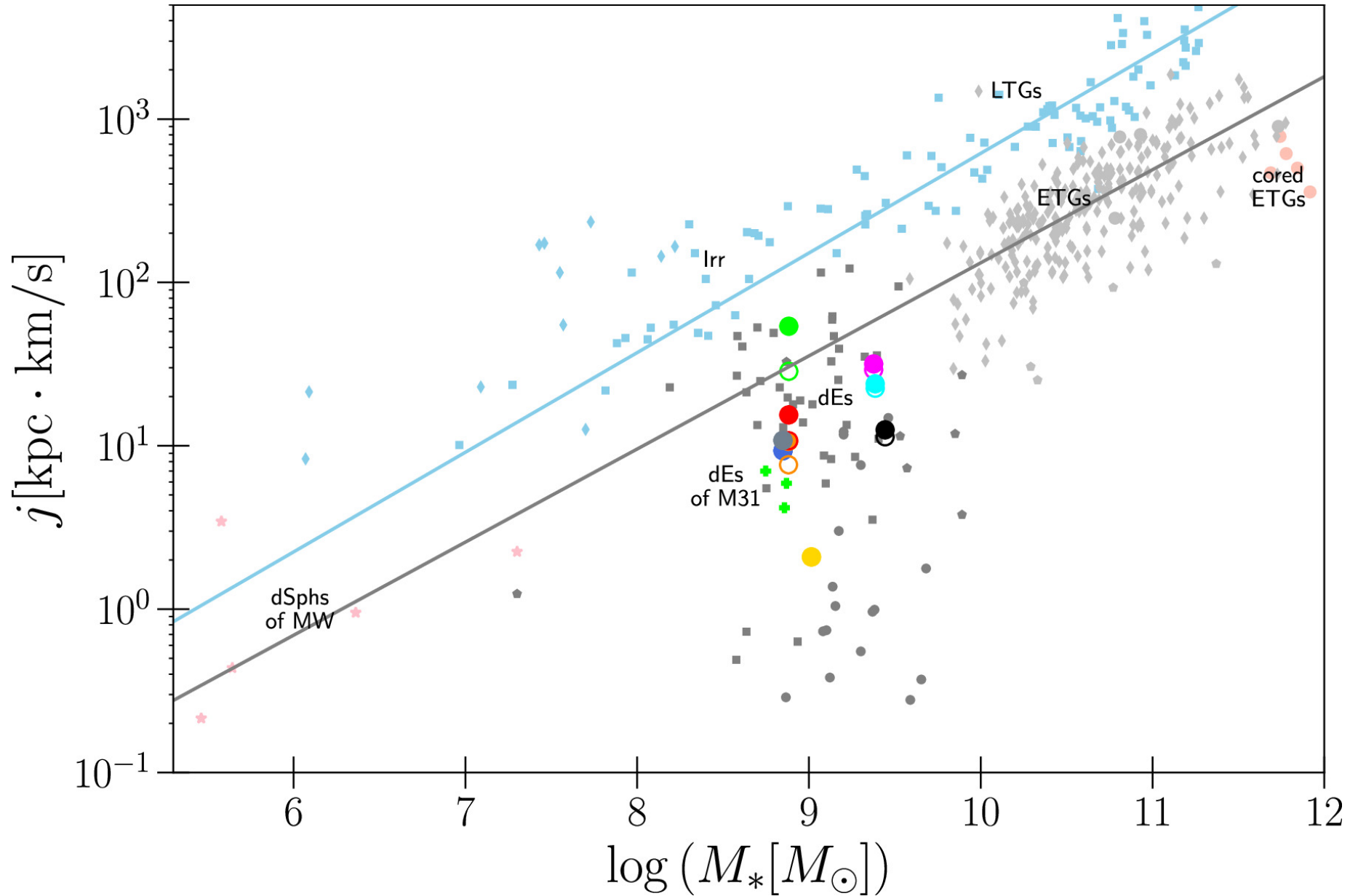
Figure 28. from Mathias Lipka et al 2024 Astrophys. J. 976 doi:10.3847/1538-4357/ad7bac https://dx.doi.org/10.3847/1538-4357/ad7bac © 2024. The Author(s). Published by the American Astronomical Society.
