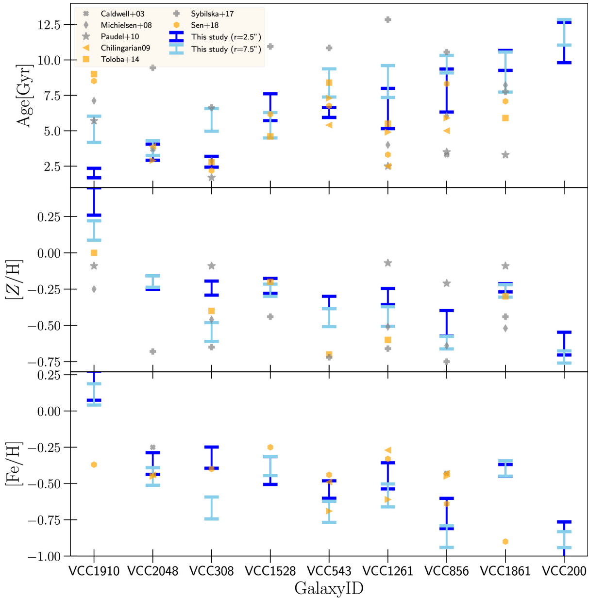
Figure 25. from Mathias Lipka et al 2024 Astrophys. J. 976 doi:10.3847/1538-4357/ad7bac https://dx.doi.org/10.3847/1538-4357/ad7bac © 2024. The Author(s). Published by the American Astronomical Society.
