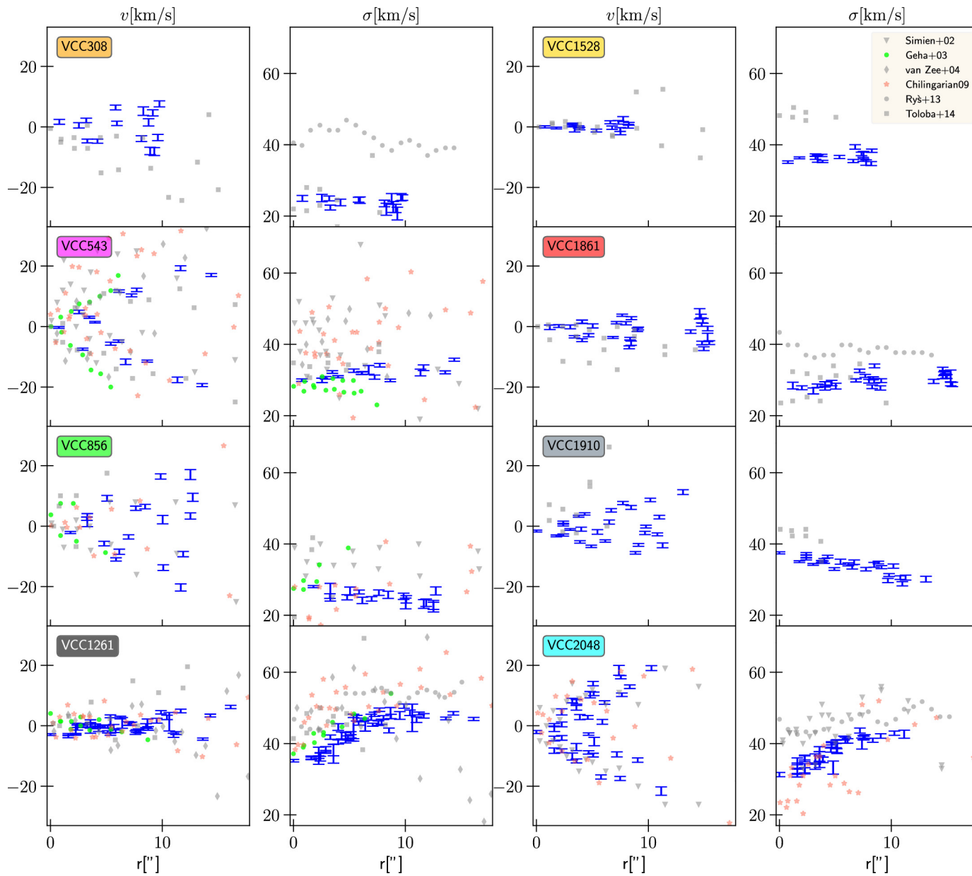
Figure 24. from Mathias Lipka et al 2024 Astrophys. J. 976 doi:10.3847/1538-4357/ad7bac https://dx.doi.org/10.3847/1538-4357/ad7bac © 2024. The Author(s). Published by the American Astronomical Society.
