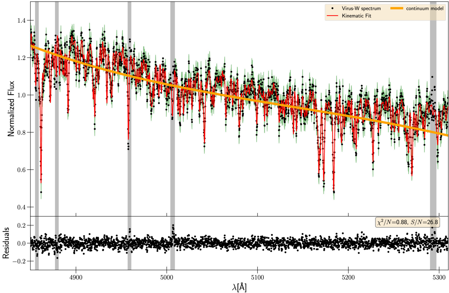
Figure 22. from Mathias Lipka et al 2024 Astrophys. J. 976 doi:10.3847/1538-4357/ad7bac https://dx.doi.org/10.3847/1538-4357/ad7bac © 2024. The Author(s). Published by the American Astronomical Society.
