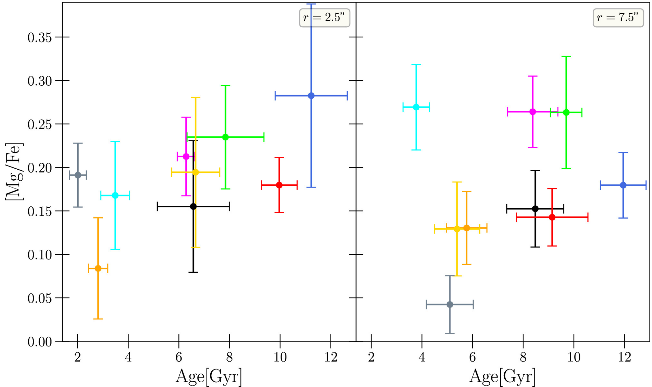
Figure 21. from Mathias Lipka et al 2024 Astrophys. J. 976 doi:10.3847/1538-4357/ad7bac https://dx.doi.org/10.3847/1538-4357/ad7bac © 2024. The Author(s). Published by the American Astronomical Society.
