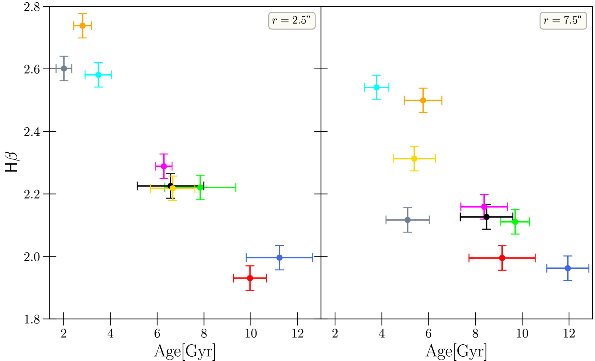
Figure 20. from Mathias Lipka et al 2024 Astrophys. J. 976 doi:10.3847/1538-4357/ad7bac https://dx.doi.org/10.3847/1538-4357/ad7bac © 2024. The Author(s). Published by the American Astronomical Society.
