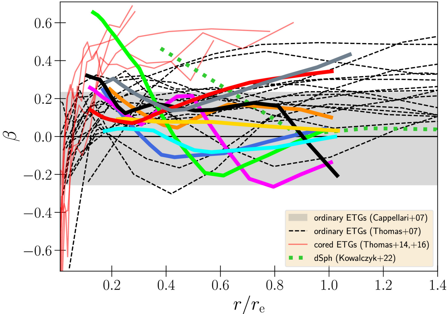
Figure 14. from Mathias Lipka et al 2024 Astrophys. J. 976 doi:10.3847/1538-4357/ad7bac https://dx.doi.org/10.3847/1538-4357/ad7bac © 2024. The Author(s). Published by the American Astronomical Society.
