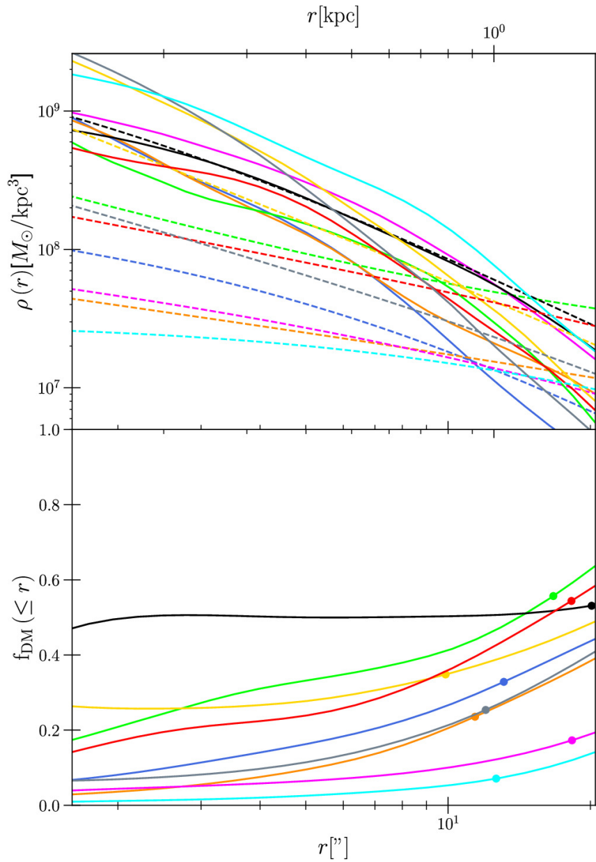
Figure 12. from Mathias Lipka et al 2024 Astrophys. J. 976 doi:10.3847/1538-4357/ad7bac https://dx.doi.org/10.3847/1538-4357/ad7bac © 2024. The Author(s). Published by the American Astronomical Society.
