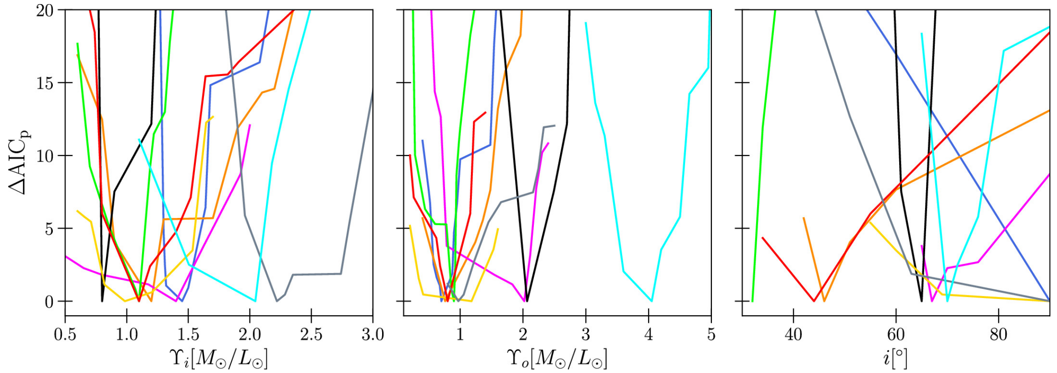
Figure 11. from Mathias Lipka et al 2024 Astrophys. J. 976 doi:10.3847/1538-4357/ad7bac https://dx.doi.org/10.3847/1538-4357/ad7bac © 2024. The Author(s). Published by the American Astronomical Society.
