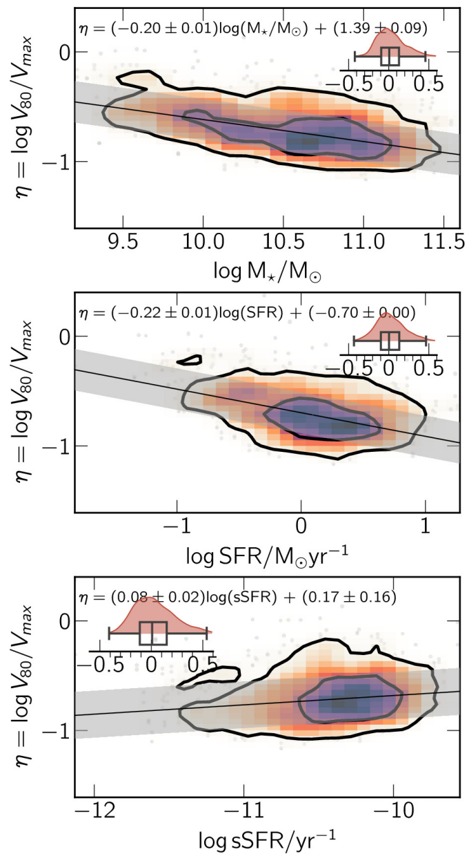
Figure 9. from Carlos López-Cobá et al 2024 Astrophys. J. 975 doi:10.3847/1538-4357/ad7b12 https://dx.doi.org/10.3847/1538-4357/ad7b12 © 2024. The Author(s). Published by the American Astronomical Society.
