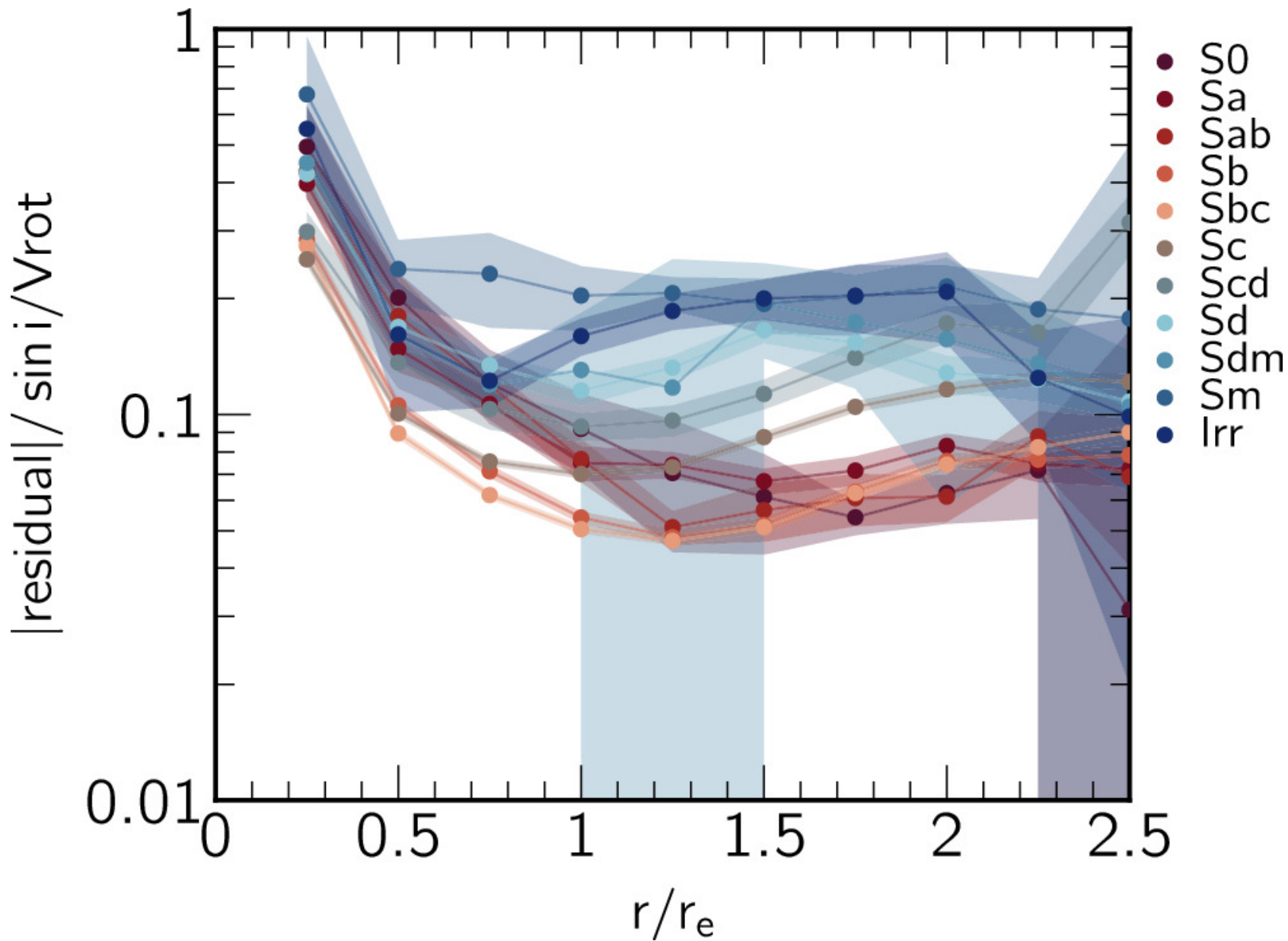
Figure 8. from Carlos López-Cobá et al 2024 Astrophys. J. 975 doi:10.3847/1538-4357/ad7b12 https://dx.doi.org/10.3847/1538-4357/ad7b12 © 2024. The Author(s). Published by the American Astronomical Society.
