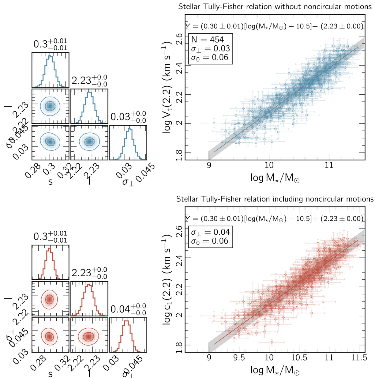
Figure 6. from Carlos López-Cobá et al 2024 Astrophys. J. 975 doi:10.3847/1538-4357/ad7b12 https://dx.doi.org/10.3847/1538-4357/ad7b12 © 2024. The Author(s). Published by the American Astronomical Society.
