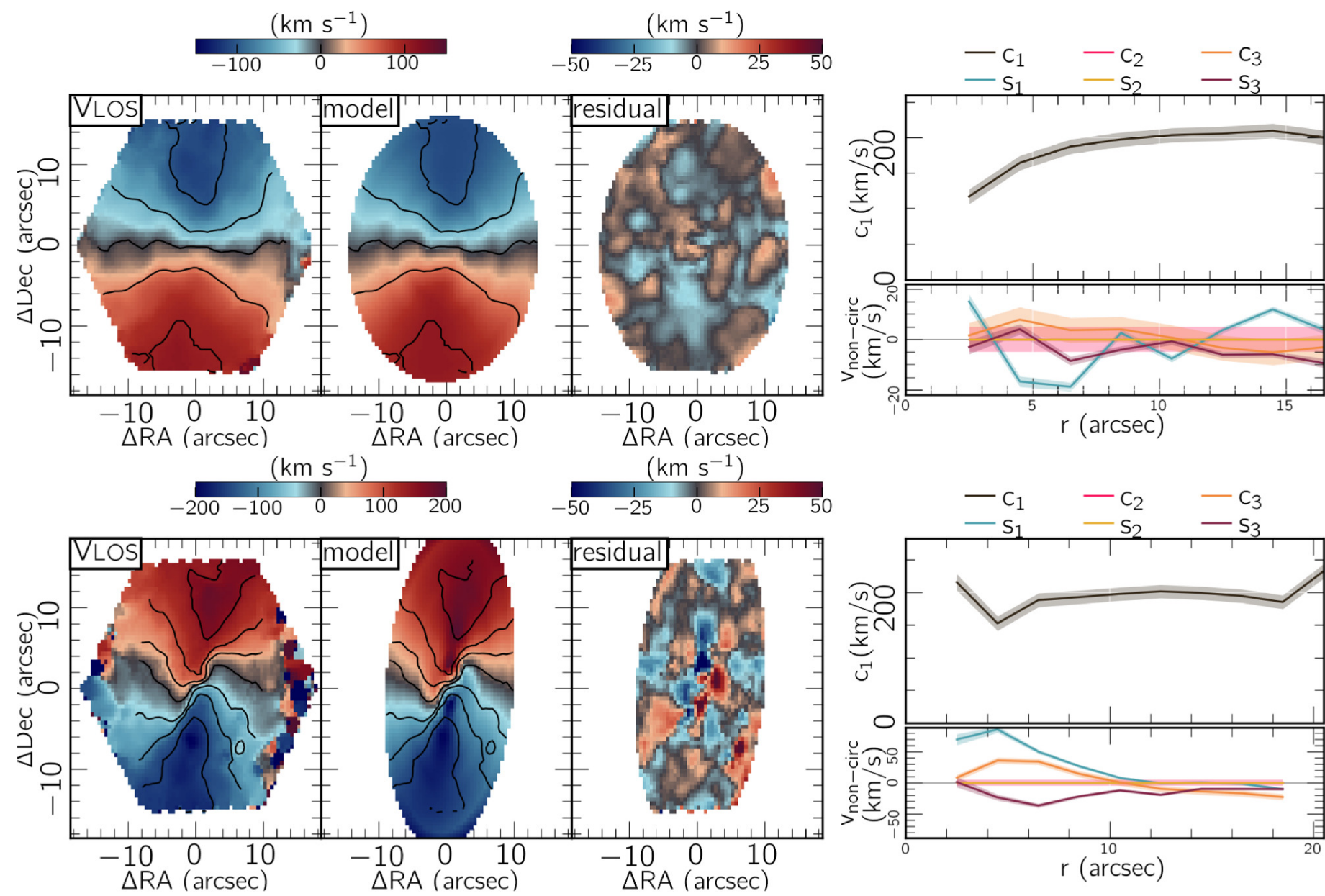
Figure 3. from Carlos López-Cobá et al 2024 Astrophys. J. 975 doi:10.3847/1538-4357/ad7b12 https://dx.doi.org/10.3847/1538-4357/ad7b12 © 2024. The Author(s). Published by the American Astronomical Society.
